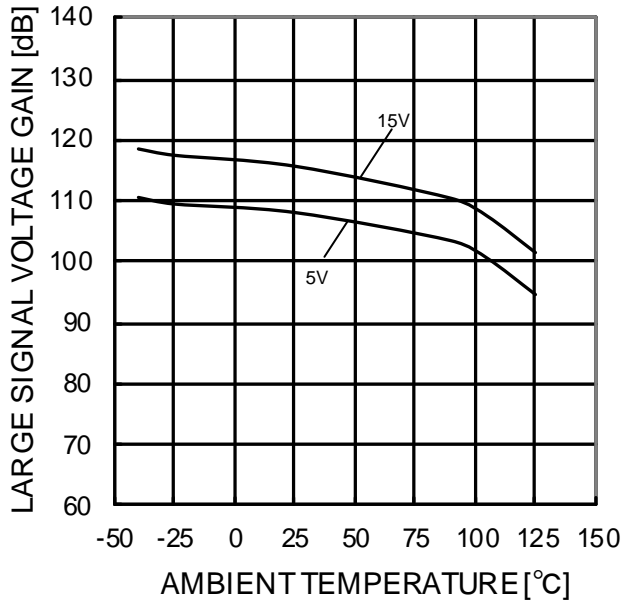
Figure 46. Large Signal Voltage Gain - Ambient Temperature ( R_L=2k\Omega )
