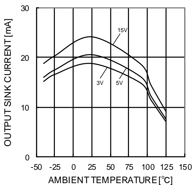
Figure 34. Output Sink Current - Ambient Temperature (OUT= V cc + )
