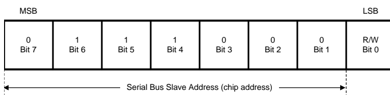
Figure 23. Chip Address
