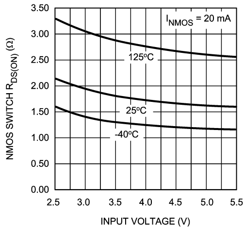
NMOS R_{DS(ON)} (Figure 1: N2) vs V_{IN}
