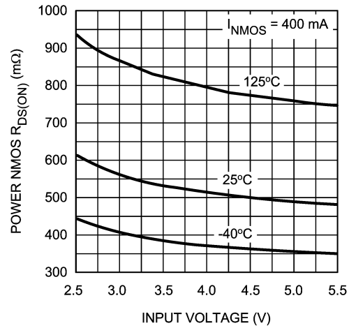
Power NMOS R_{DS(ON)} (Figure 1: N1) vs V_{IN}
