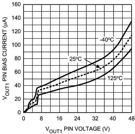
V_{OUT1} Pin Current vs V_{OUT1} Pin Voltage
