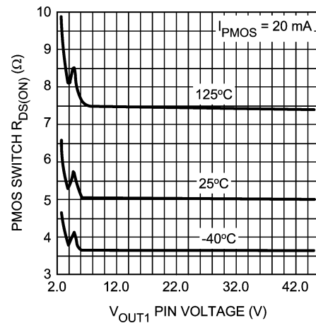
PMOS R_{DS(ON)} (Figure 1: P1) vs V_{IN}
