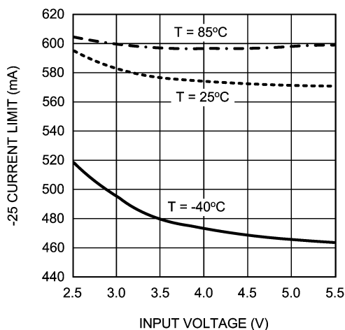
Current Limit (LM3503-25) vs V_{IN}
