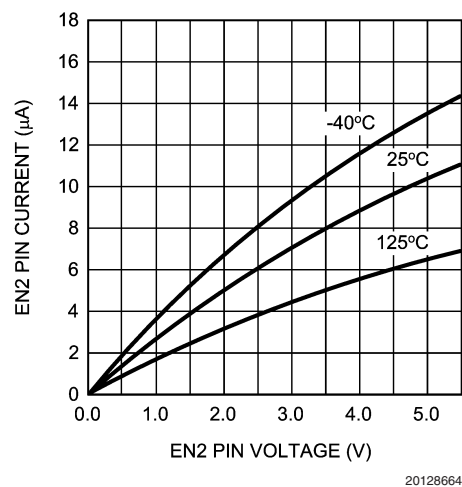
En2 Pin Current vs En2 Pin Voltage
