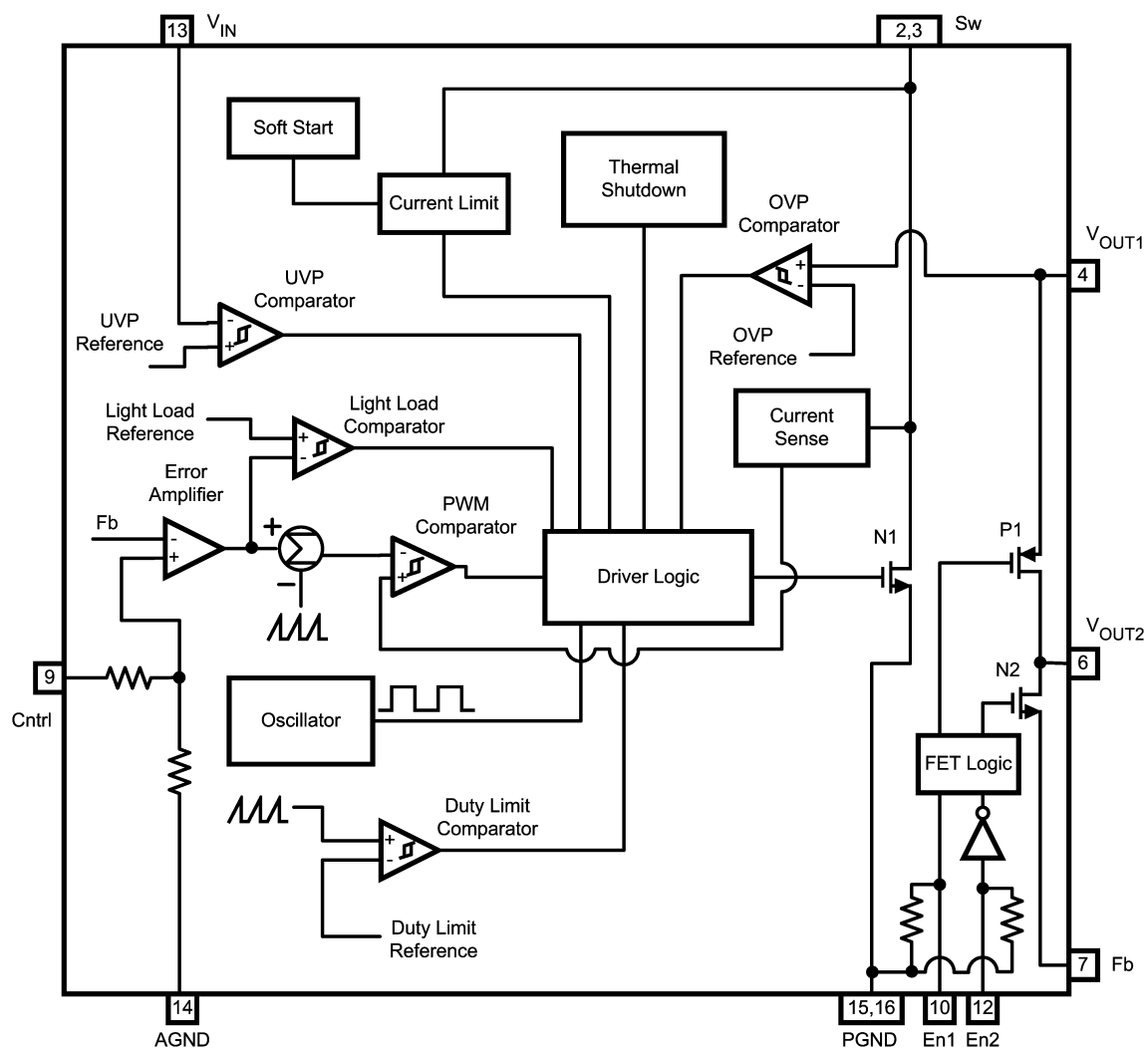
FIGURE 1. Block Diagram
