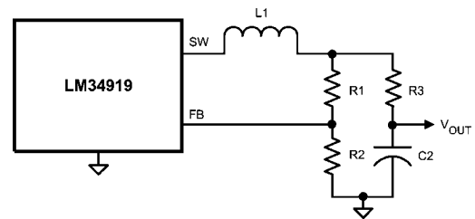
FIGURE 10. Alternate Minimum Output Ripple Configuration
