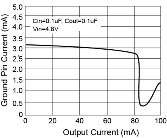
FIGURE 5. Ground Pin Current versus Output Current
