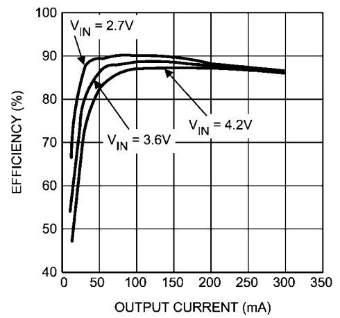
Efficiency vs Output Current ( V_{OUT} = 1.5\text{V} )
