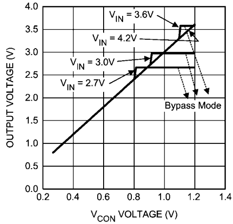
V CON Voltage vs PWM Output Voltage ( I_{OUT} = 200\text{mA} )
