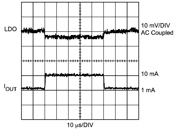
LDO Load Transient Response ( C_{OUT} = 1 \mu F )
