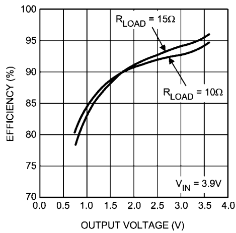
Efficiency vs Output Voltage ( V_{IN} = 3.9\text{V} )
