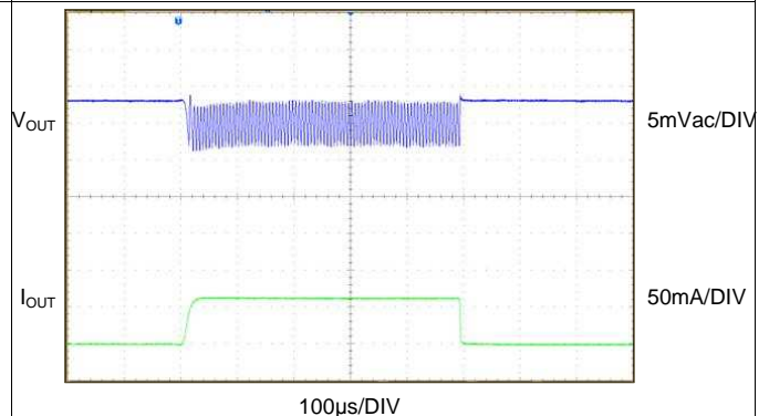
Figure 10. V_{OUT} Transient
