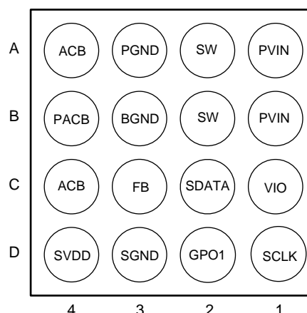
YFQ Package 16-Pin DSBGA Bottom View
