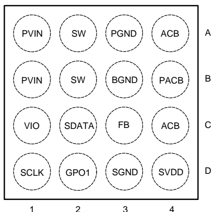
YFQ Package 16-Pin DSBGA Top View
