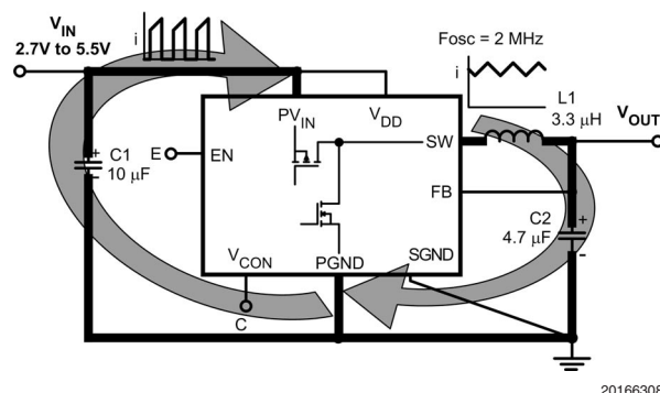
FIGURE 4. Current Loop
