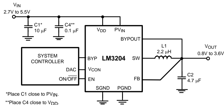
Figure 3. Typical Operating System Circuit
