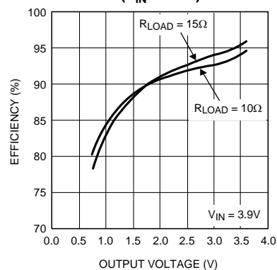
Efficiency vs Output Voltage ( V_{IN} = 3.9V )
