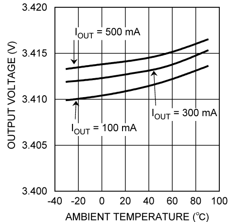
Output Voltage vs Temperature ( V_{IN} = 4.2V , V_{OUT} = 3.4V , V_{CON} = 1.13V )
