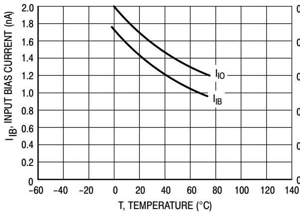
Figure 1. Input Bias and Input Offset Currents
