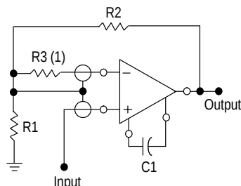
Noninverting Amplifier
