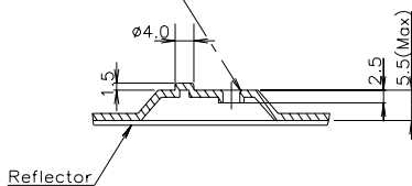
SECTION B-B SCALE 1/1(2ea)
