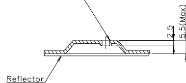
SECTION C-C SCALE 1/1(6ea)
