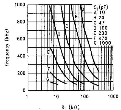
FIGURE 1. Frequency vs R_T and C_T Graph
