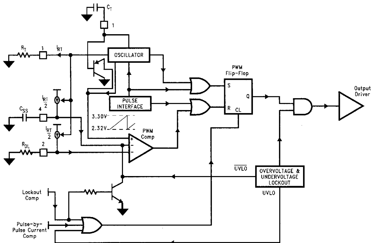
FIGURE 2. PWM Block Diagram
