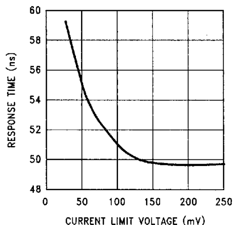
FIGURE 16. Current Limit Response Time
