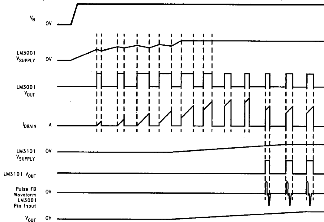
FIGURE 11. Start-Up Timing Sequence
