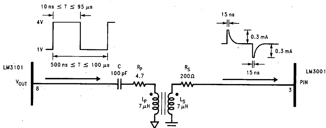
FIGURE 15. Pulse Interface Circuit
