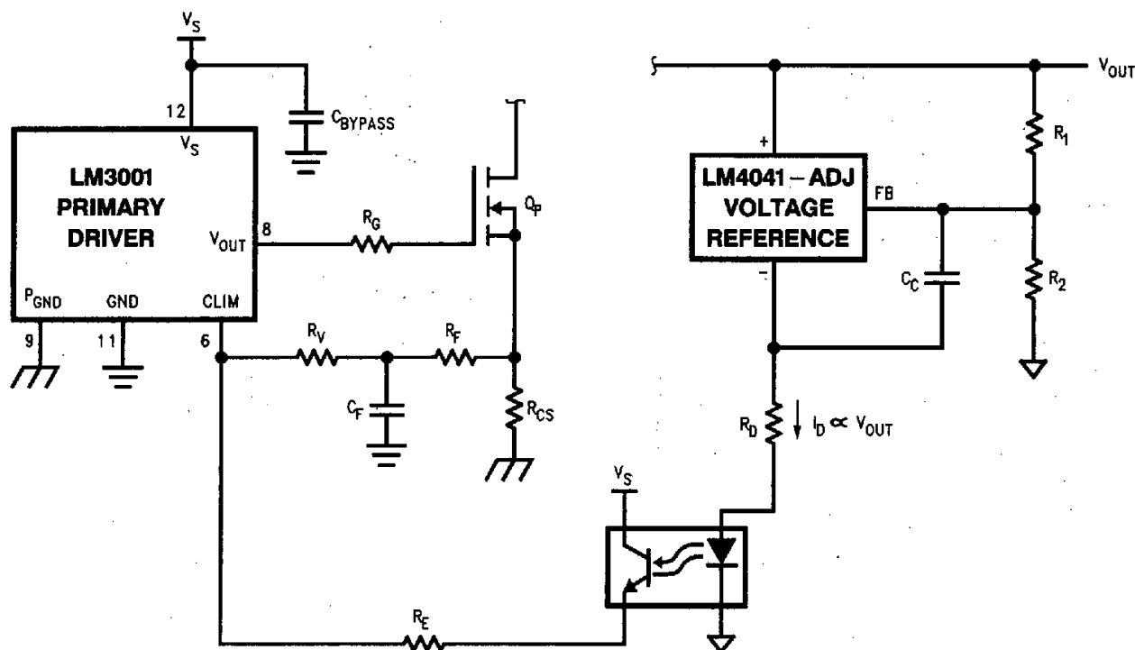
FIGURE 17. Opto-Coupler Feedback Circuit
