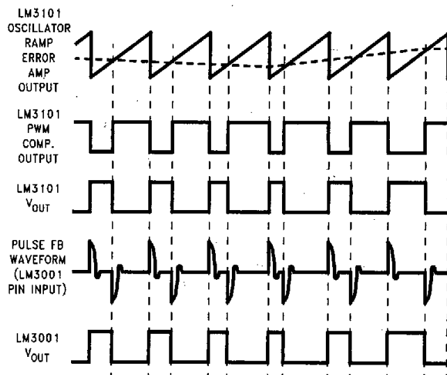
FIGURE 14. Pulse Feedback Timing Diagram
