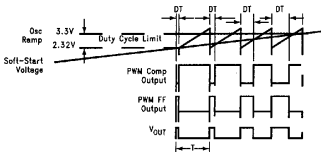
FIGURE 4. Soft-Start Timing Diagram
