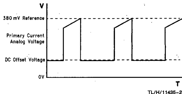
FIGURE 18. Opto-Coupler Feedback Waveforms
