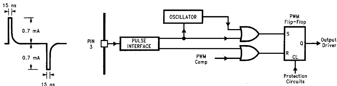
FIGURE 5. Pulse Interface Block Diagram
