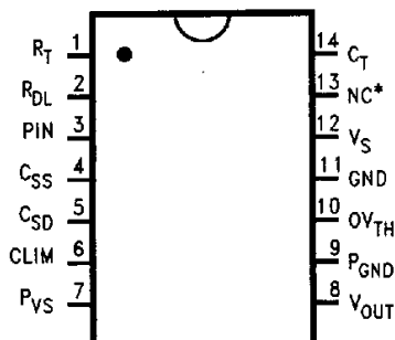
14-Lead Package
