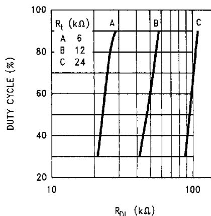
FIGURE 3. Maximum Duty Cycle vs R_{DL}
