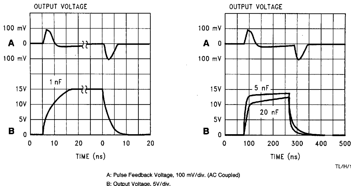
FIGURE 6. Output Voltage Rise and Fall Times
