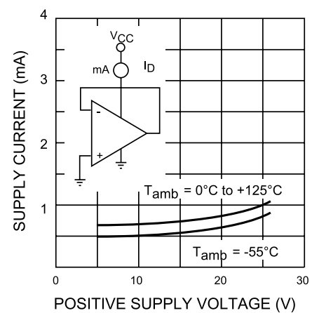
Figure 6. Supply current
