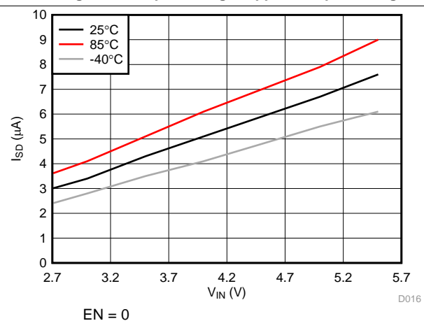
Figure 4. Shutdown Current
