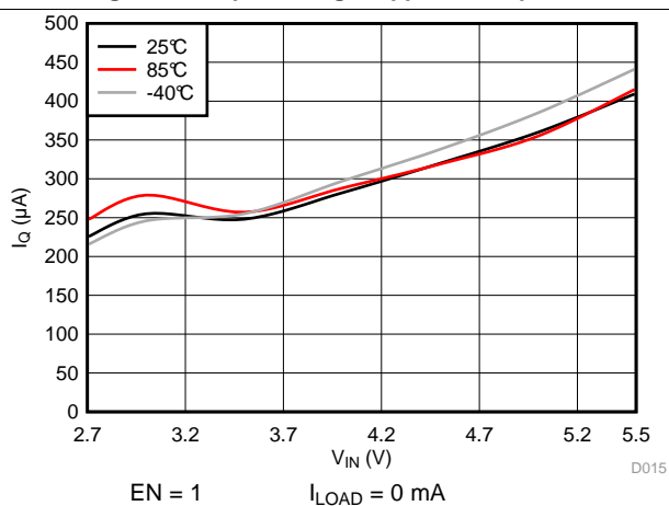
Figure 3. Quiescent Current
