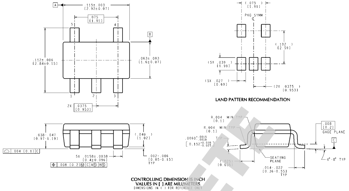
5 Lead Small Outline Package (SOT-23-5) MS05A
