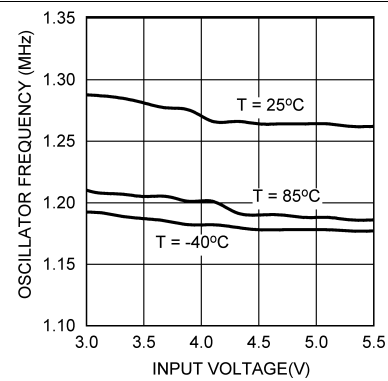
Figure 14. Oscillator Frequency vs. Input Voltage
