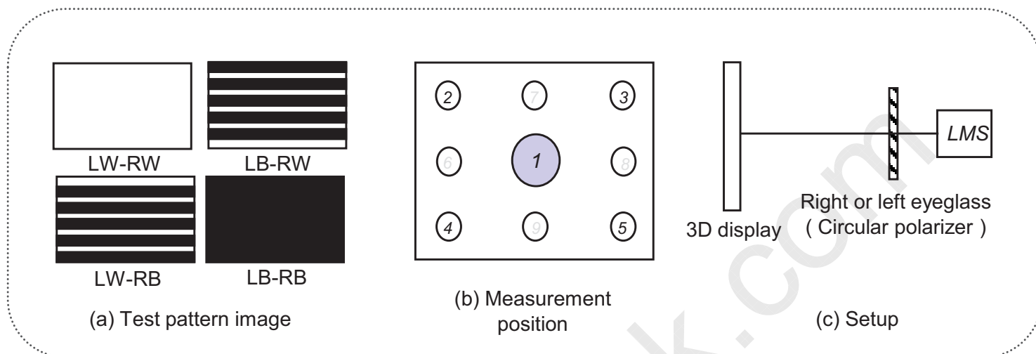
Figure 15. Measurement configuration
