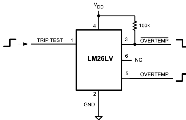
FIGURE 8. TRIP TEST Digital Output Test Circuit
