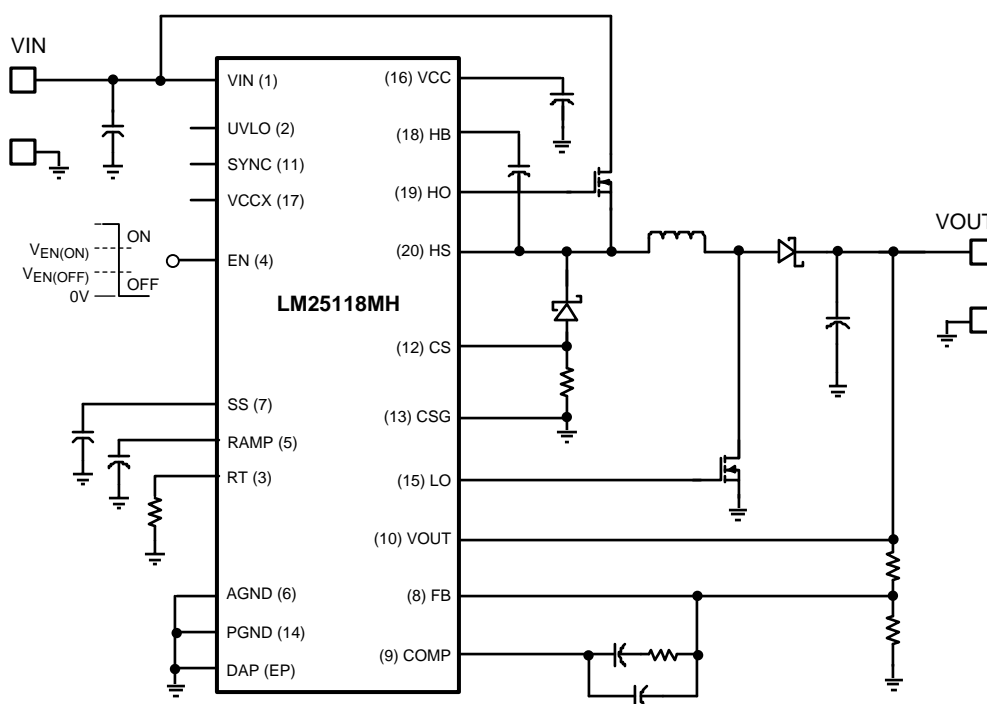
Figure 18. Typical Application Circuit
