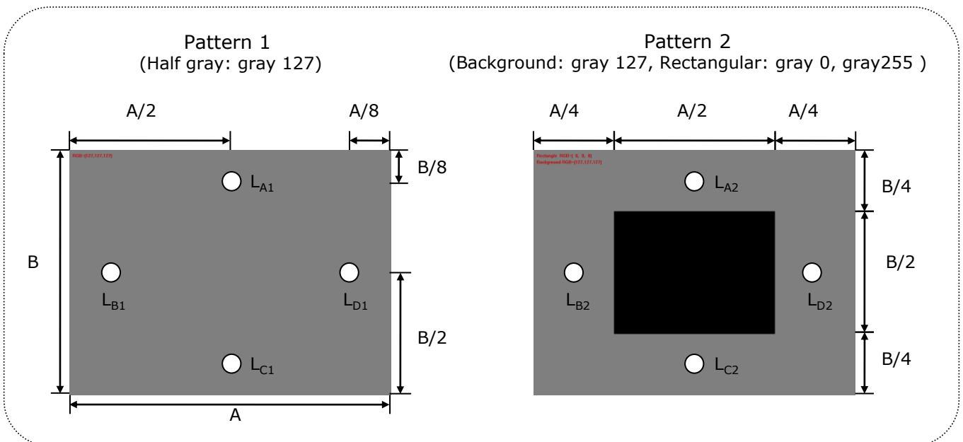
FIG. 11 Crosstalk
