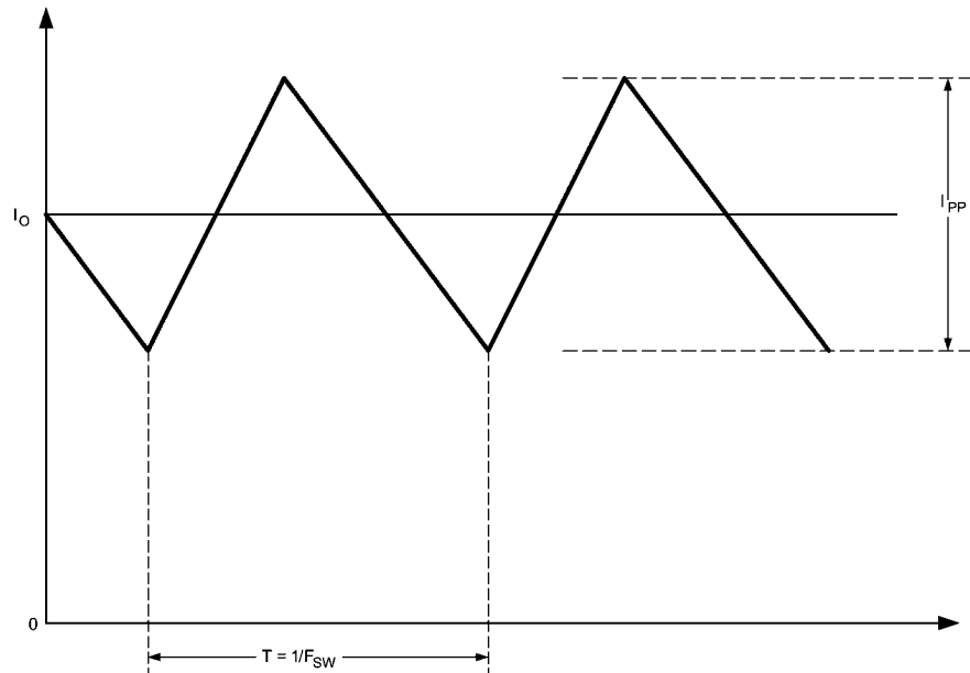
FIGURE 9. Inductor Current
