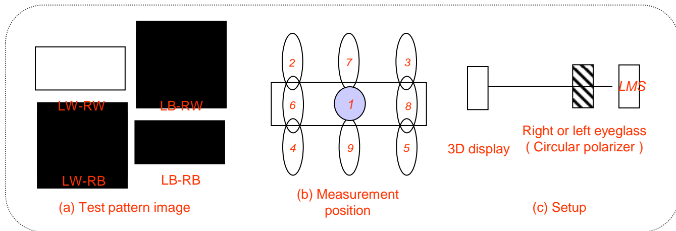
Figure 14. Measurement configuration
