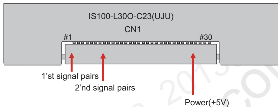
Rear view of LCM
