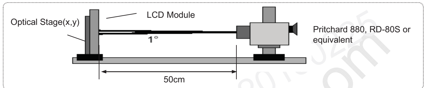
FIG. 7 Optical characteristic measurement equipment and method
