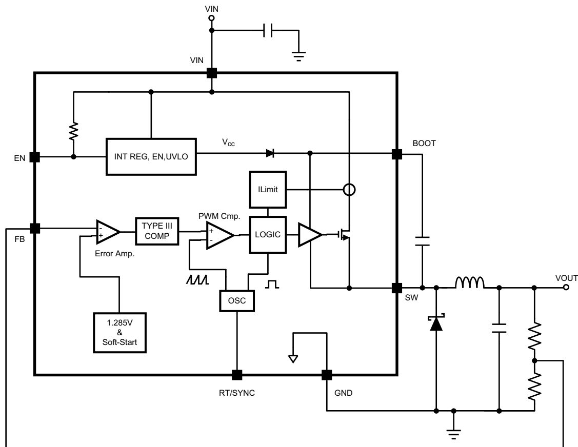
Figure 12. Simplified Block Diagram
