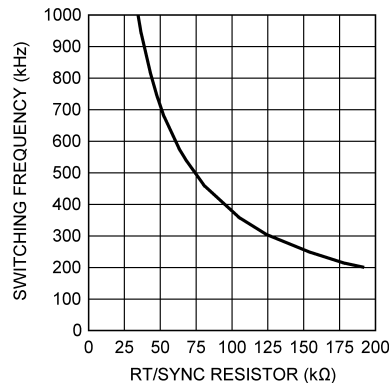
Figure 17. Switching Frequency vs RT/SYNC Resistor
