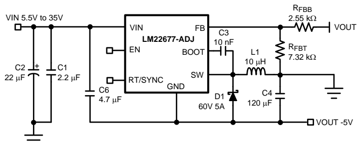
Figure 23. Inverting Regulator Application
