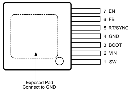
Figure 1. 7-Lead Plastic PFM Package Package Number NDR0007A
