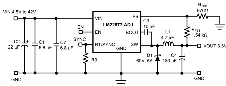
Figure 20. Typical Buck Regulator Application
