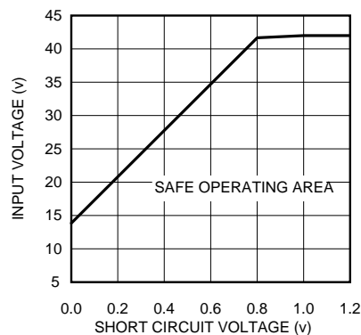
Figure 16. SOA at 800 kHz
