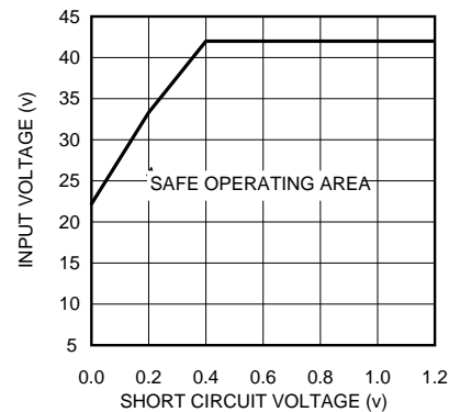
Figure 15. SOA at 500 kHz
