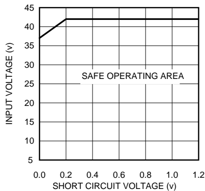
Figure 14. SOA at 300 kHz
