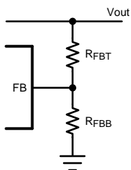
Figure 21. Resistive Feedback Divider
