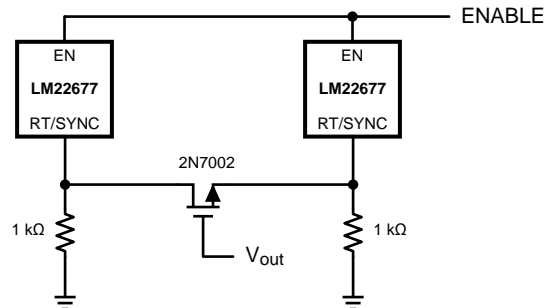
Figure 18. Self Synchronizing Setup
