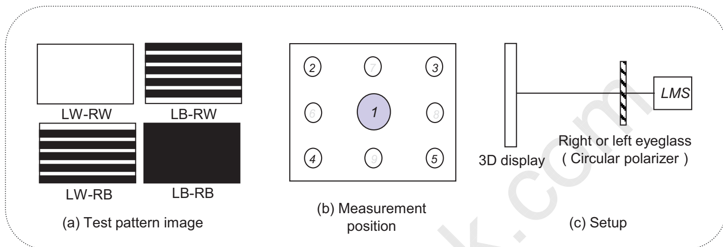
Figure 13. Measurement configuration
