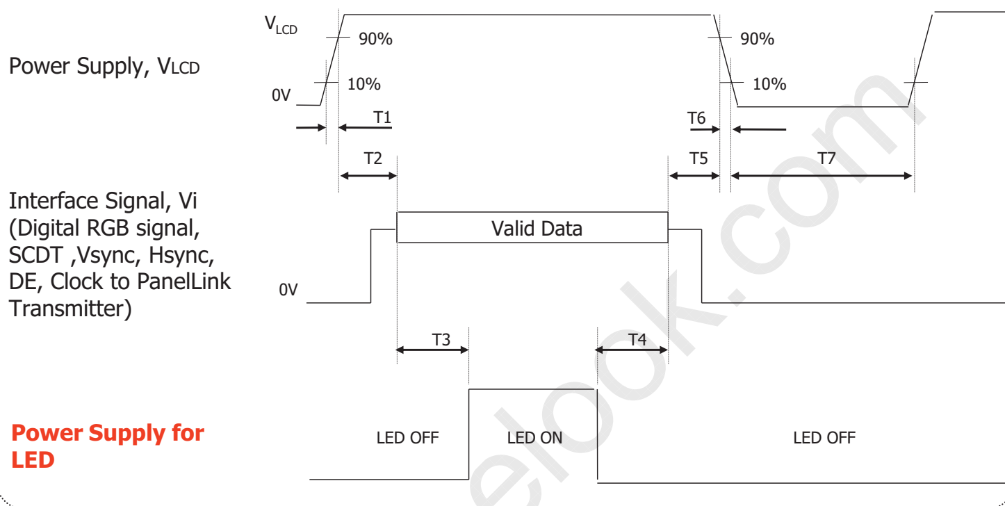
FIG.5 Power sequence
