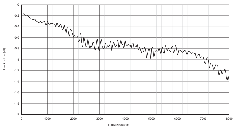
Insertion Loss vs. Frequency
