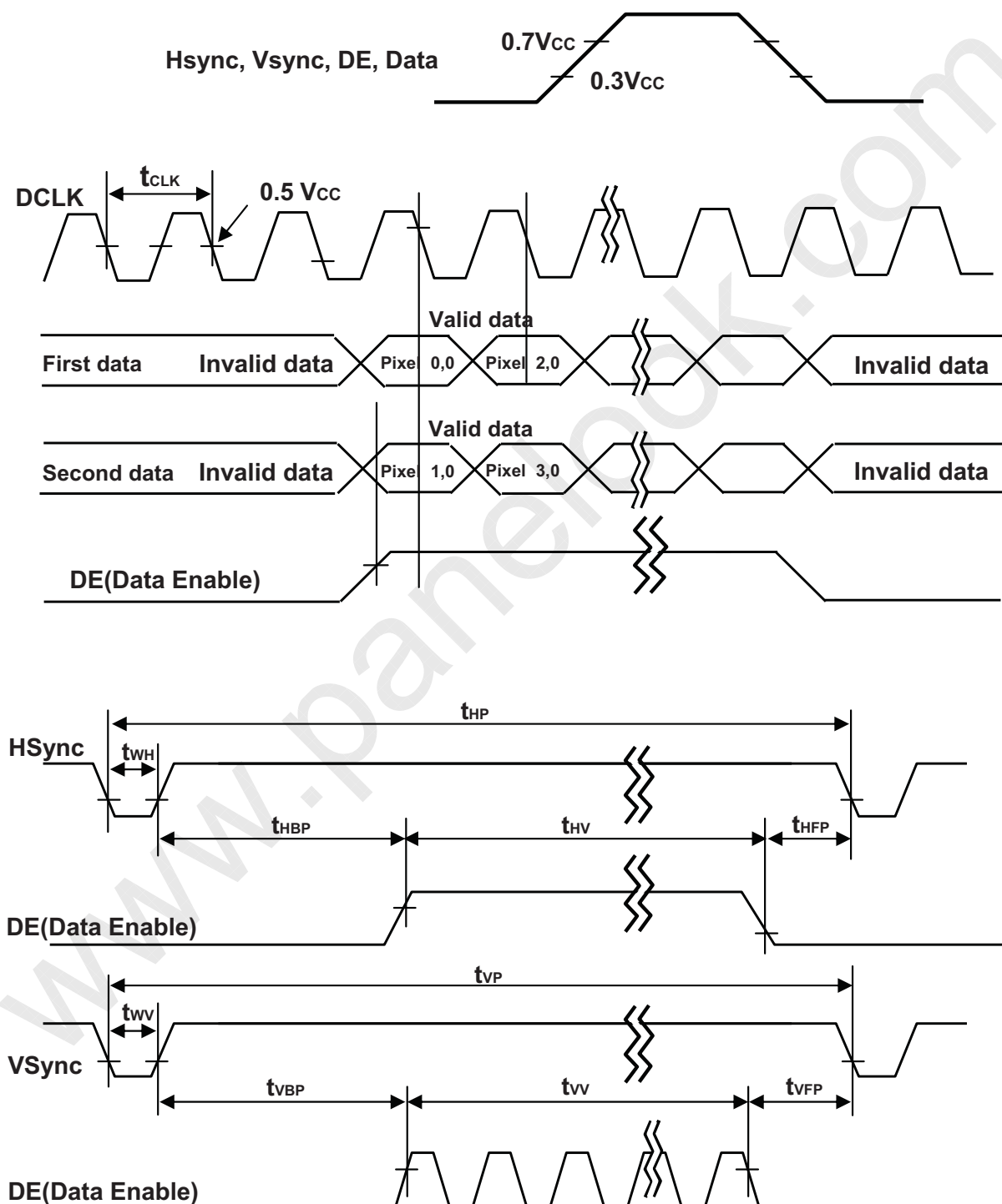
[ Figure 6 ] Signal timing waveforms
