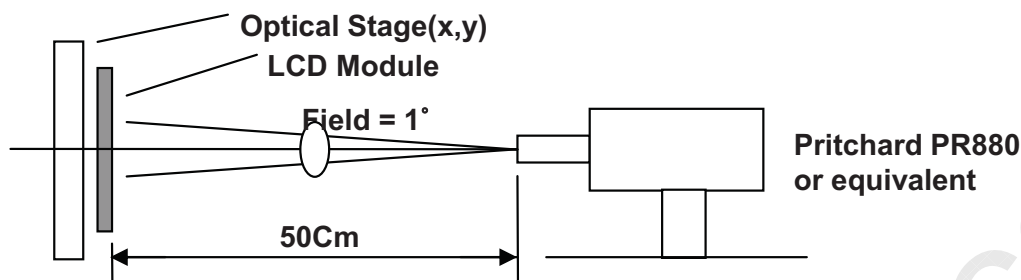
[Figure 9] Optical characteristic measurement equipment and method
