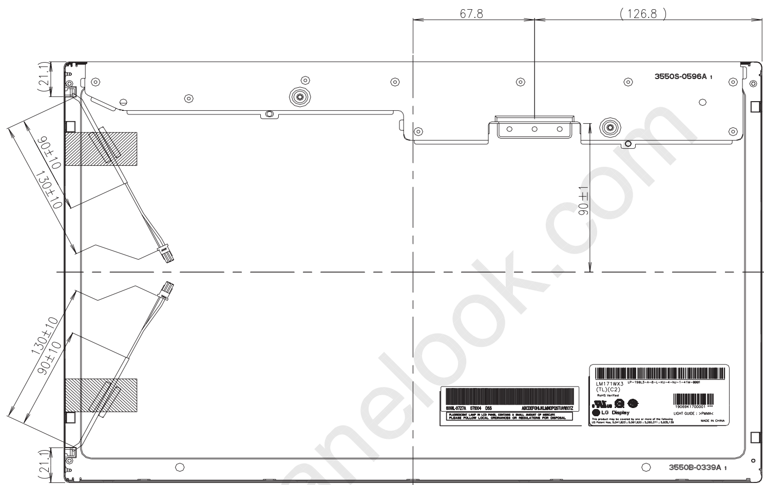
Figure 15. Rear view
