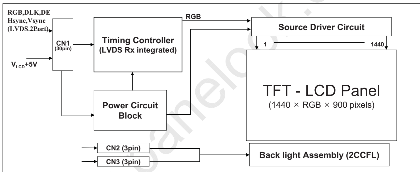
Figure 1. Block diagram
