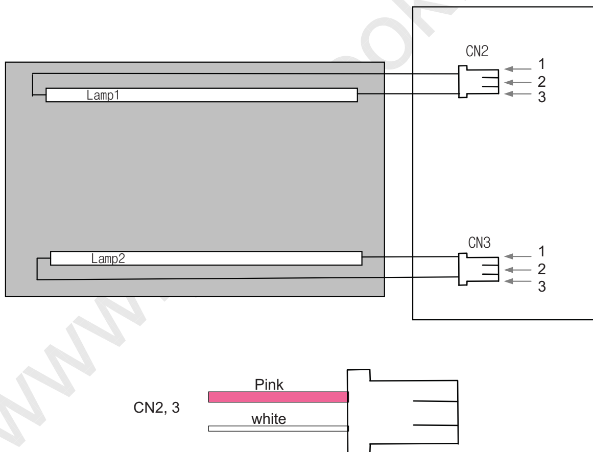
[ Figure 5 ] Backlight connector view
