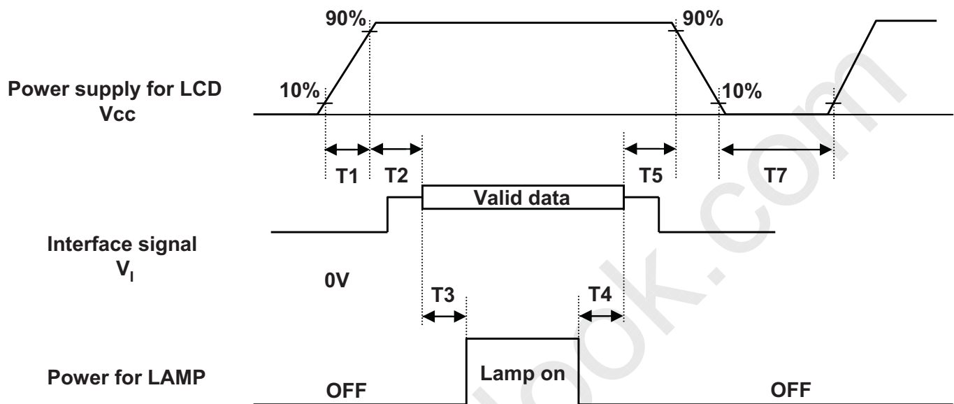
[ Figure 7 ] Power sequence
