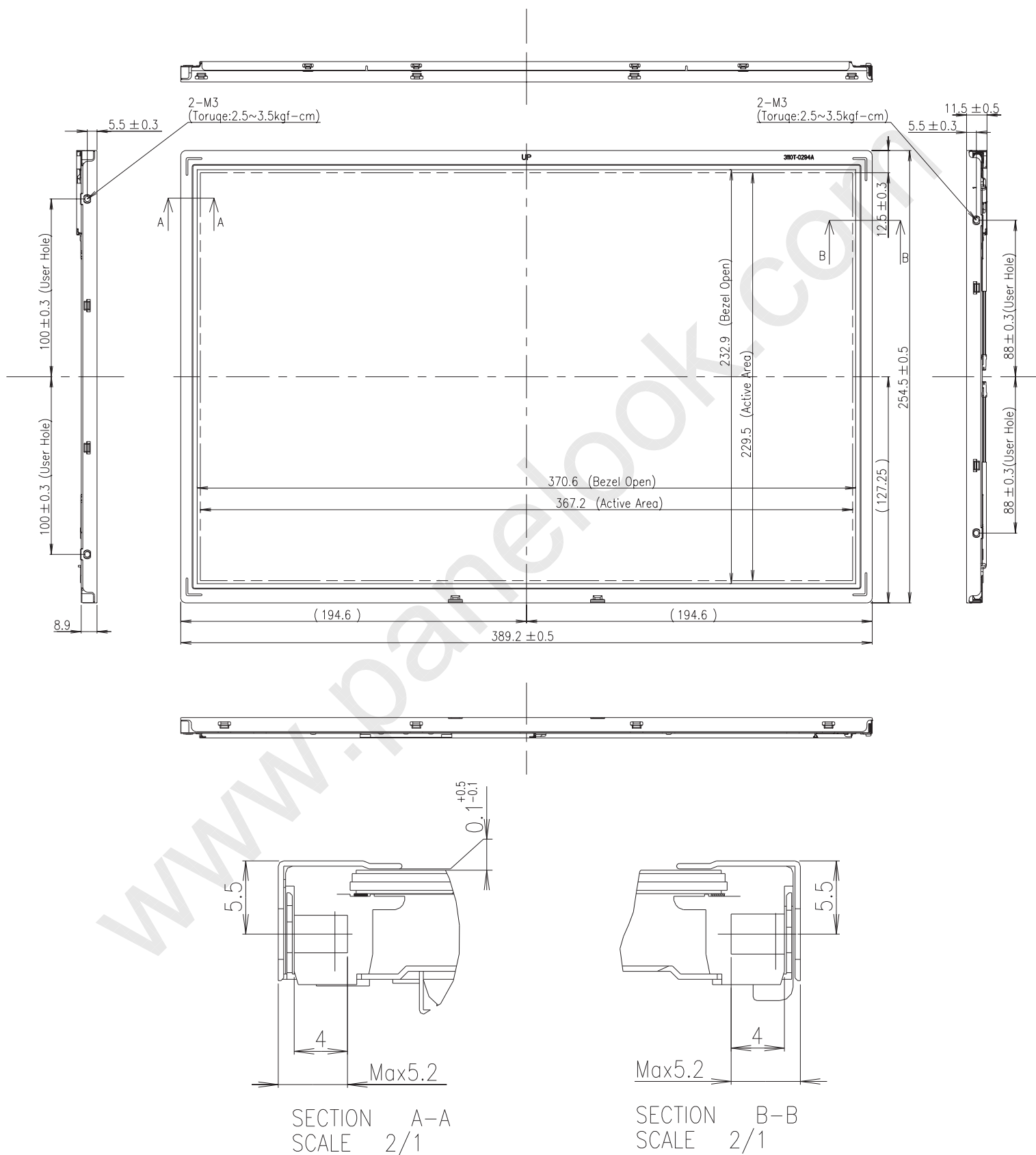
Figure 14. Front view
