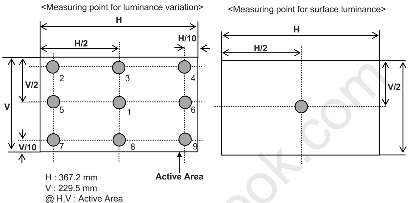
Figure 10. Luminance measuring point
