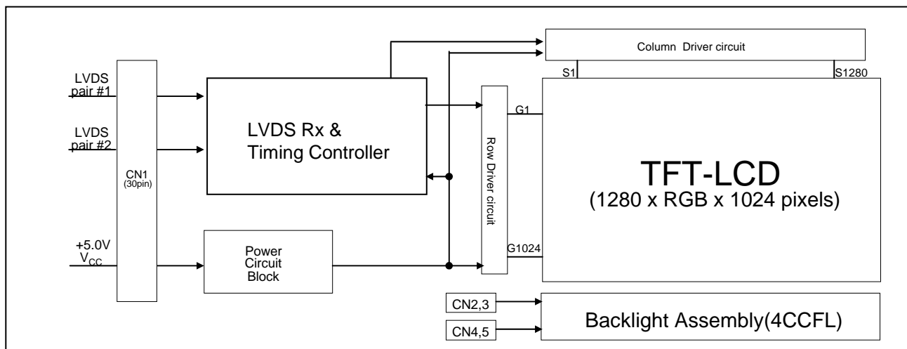
Figure 1. Block diagram
