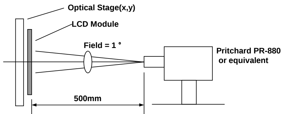
[Figure 11] Optical Characteristic Measurement Equipment and Method
