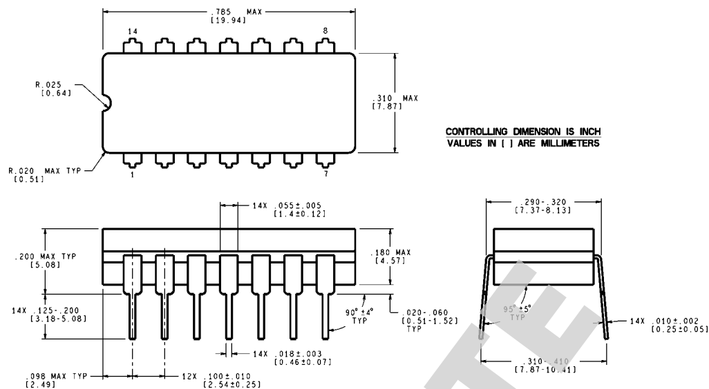
Ceramic Dual-In-Line Package NS Package Number J14A
