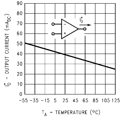
Current Limiting
