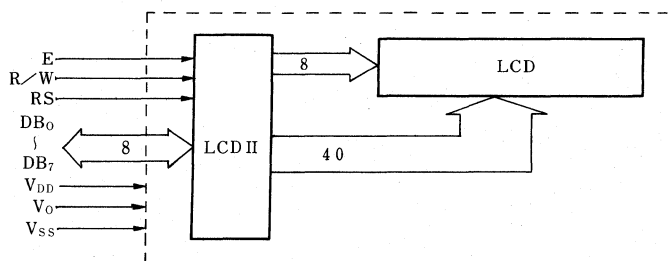
Fig. 3 Block diagram
