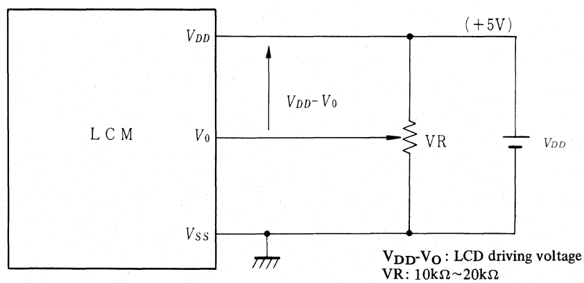
Fig. 4 Power supply
