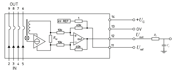
Figure 29: Filtered U_{out} connection
