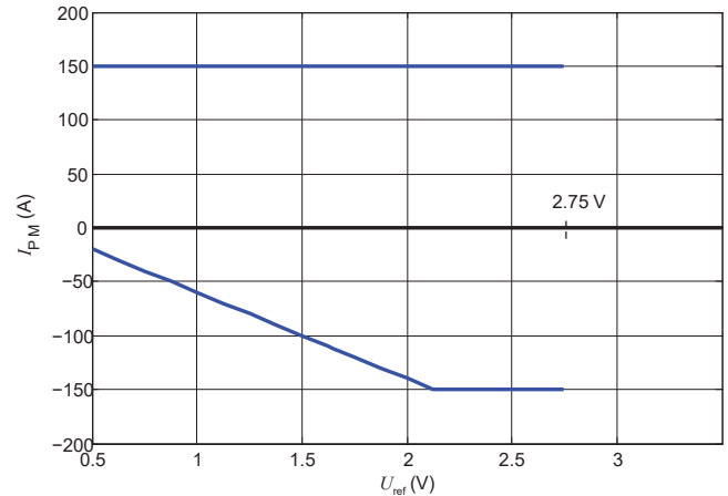
Figure 33: Measuring range versus external U_{ref} LKSR 50 A
