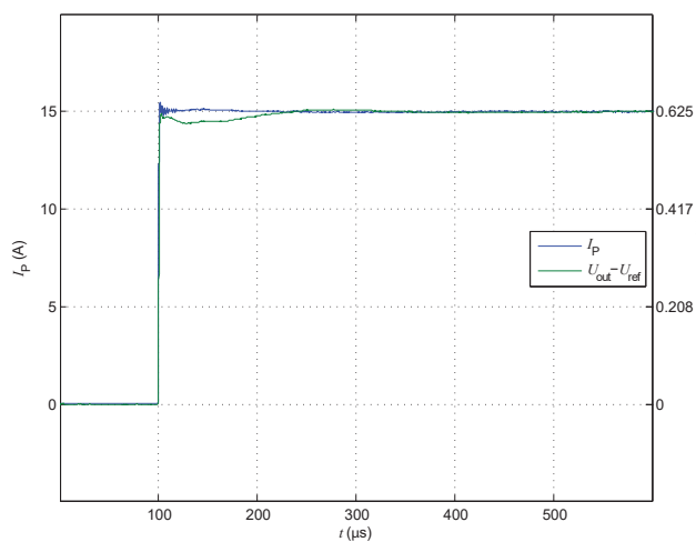
Figure 8: Delay time
