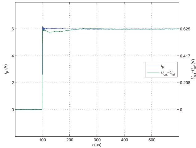
Figure 3: Delay time
