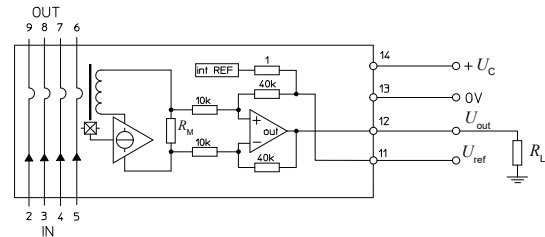
Figure 26: Test connection
