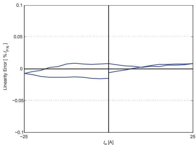
Figure 11: Linearity error
