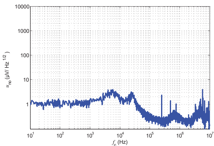
Figure 19: Noise voltage spectral density
