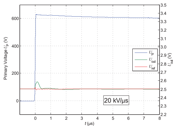
Figure 15: du/dt
