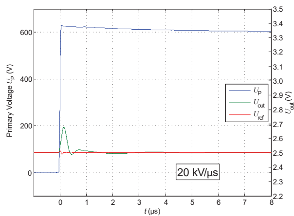
Figure 10: du/dt
