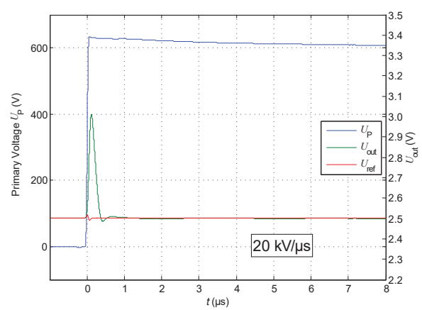
Figure 5: du/dt
