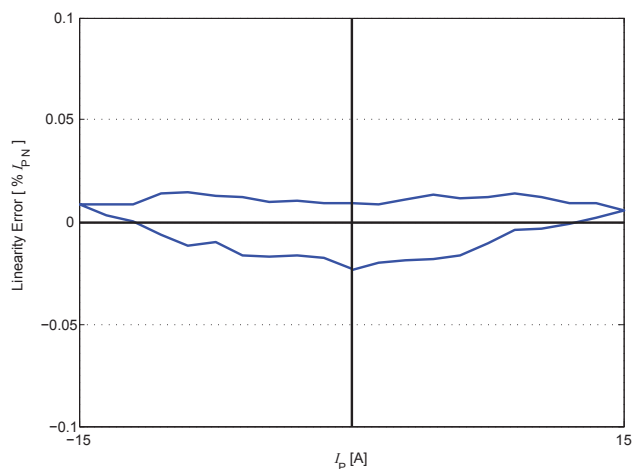
Figure 6: Linearity error
