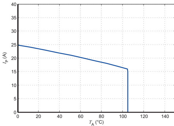
Figure 21: I_p vs T_A for LKSR 6-NP
