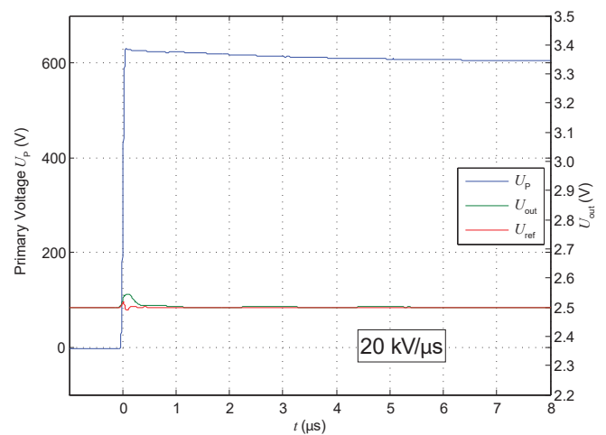
Figure 20: du/dt
