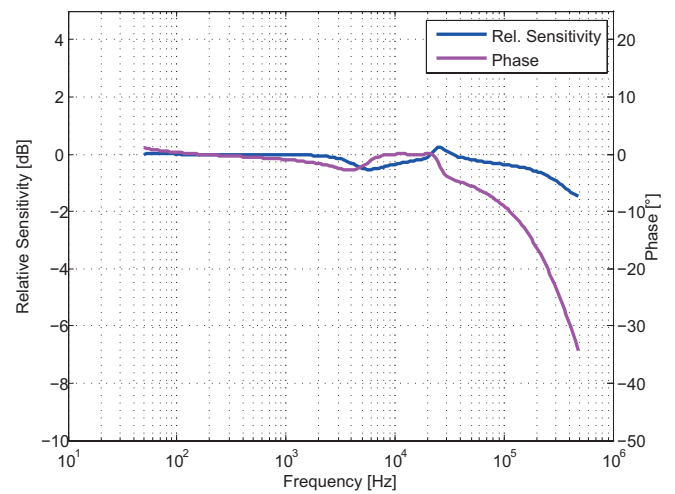
Figure 17: Frequency response
