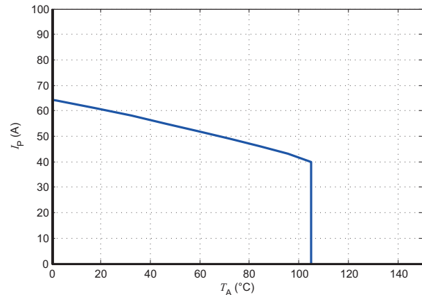
Figure 22: I_p vs T_A for LKSR 15-NP
