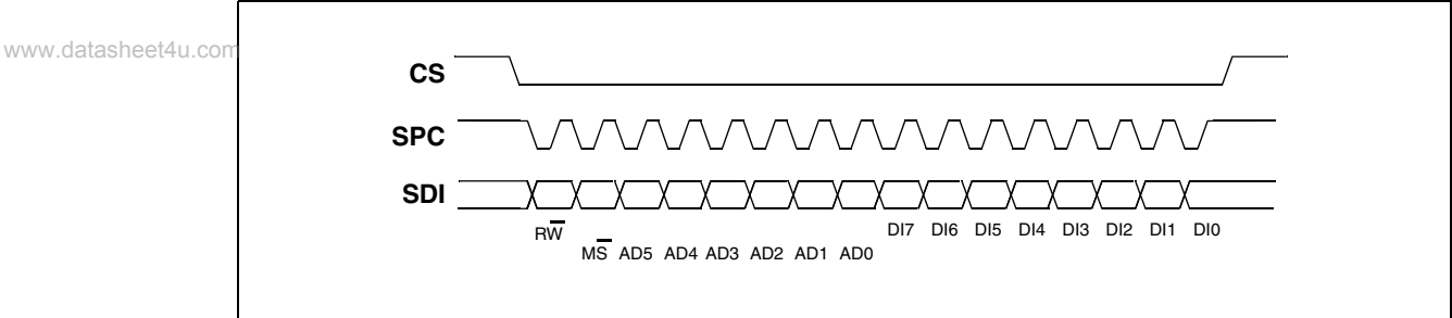
Figure 7. SPI Write protocol
