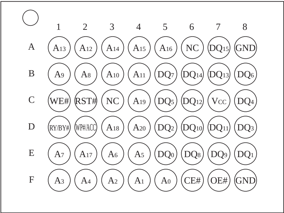
0.8mm pitch 48-BALL CSP PINOUT 8mm x 6mm TOP VIEW
