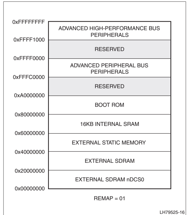
Figure 4. Memory Remap '01'
