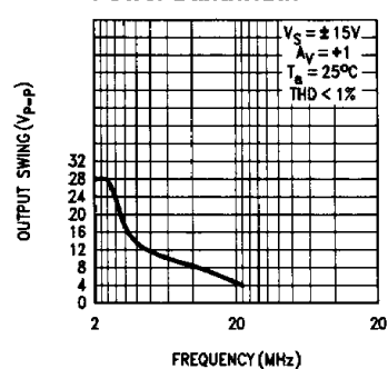
Power Bandwidth
