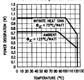
Power Dissipation Curve
