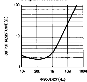
Output Resistance
