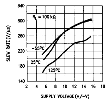
Positive Slew Rate
