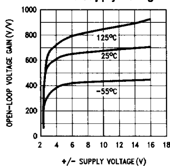
Gain vs Supply Voltage
