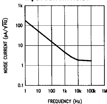
Input Current Noise
