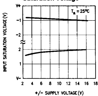
Common-Mode Input Saturation Voltage
