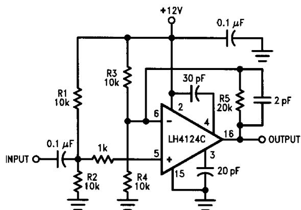
Video Amplifier
