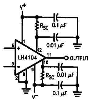
FIGURE 4. Using Resistor Current Limiting*
