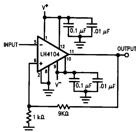
FIGURE 6. 10X Buffer Amplifier*
