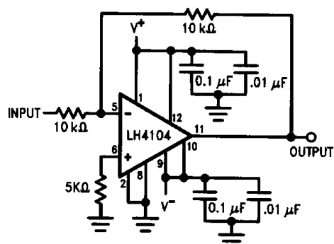
FIGURE 7. Unity Gain Inverter*
