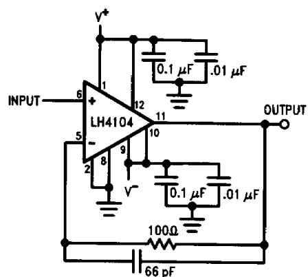
FIGURE 5. Unity Gain Follower*
