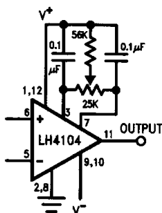
FIGURE 3. Offset Null*
