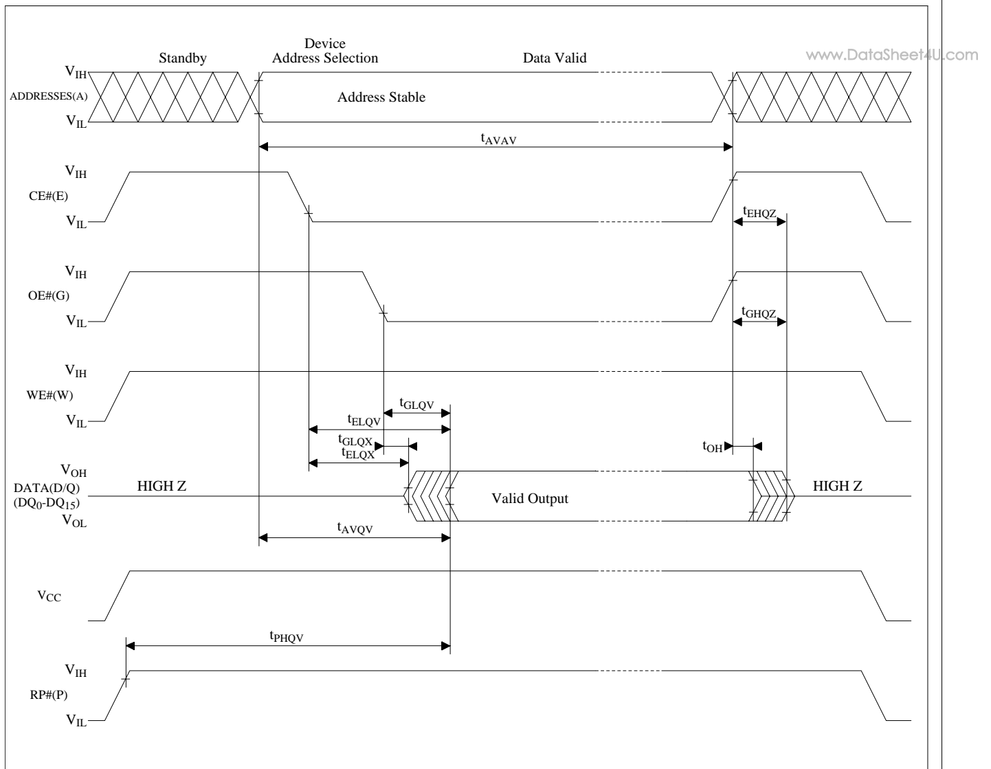
Figure 14. AC Waveform for Read Operations
