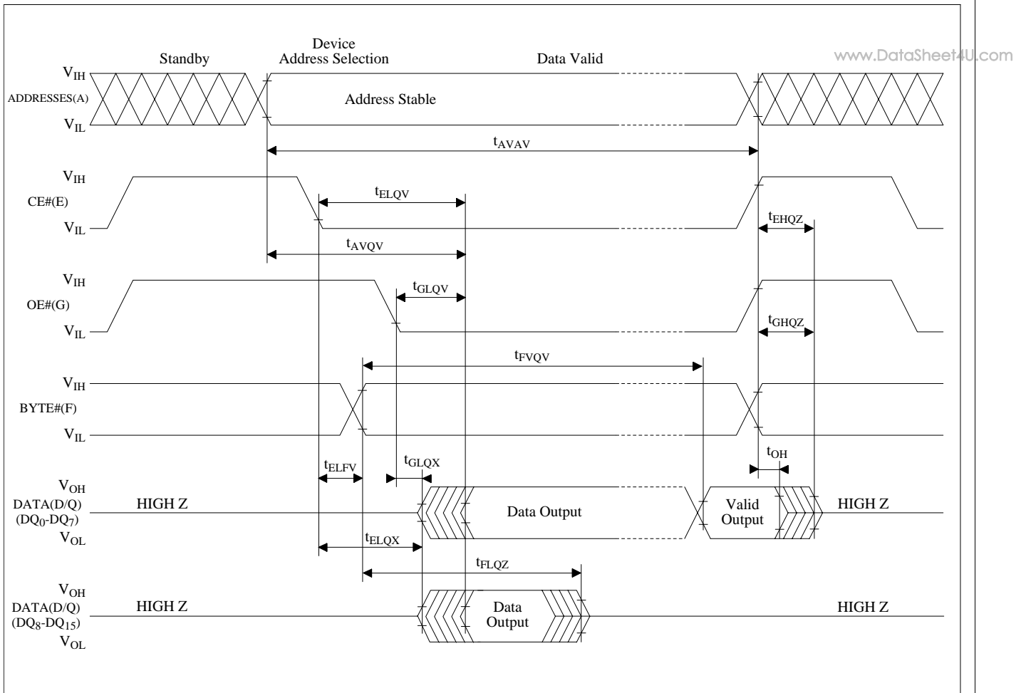
Figure 15. BYTE# timing Waveform
