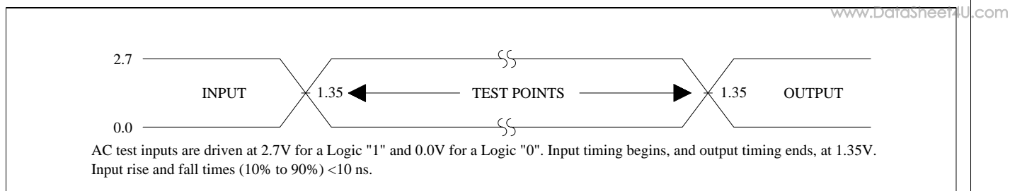
Figure 12. Transient Input/Output Reference Waveform for V_{CC}=2.7V-3.6V
