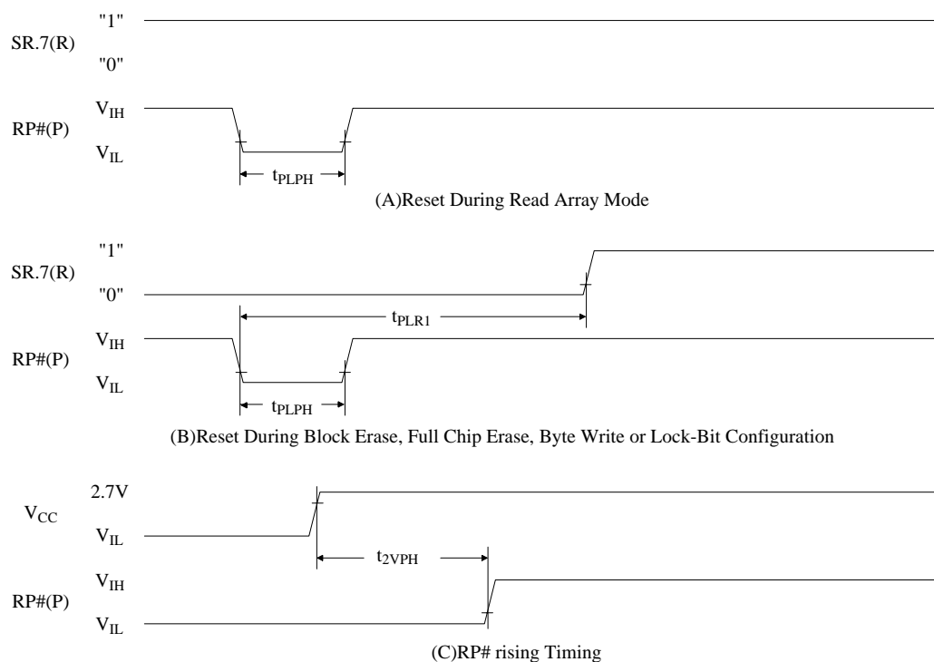
Figure 17. AC Waveform for Reset Operation
