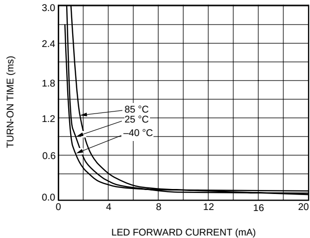
B. Turn-On Time vs. LED Current (LH1525)
