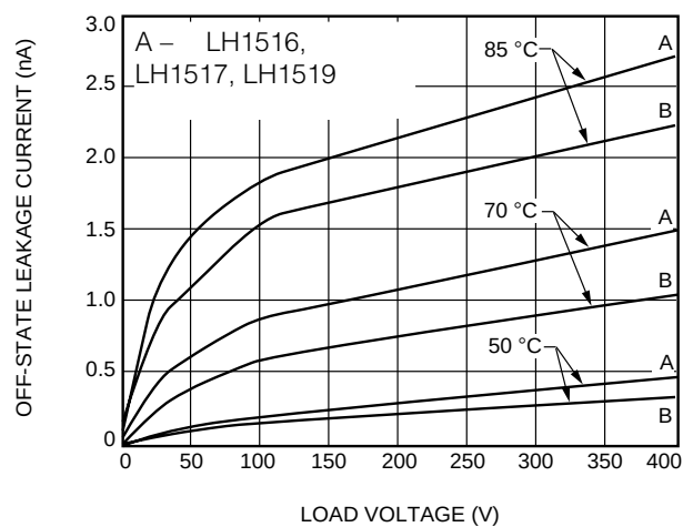
F. Leakage Current vs. Applied Voltage at Elevated Temperatures
