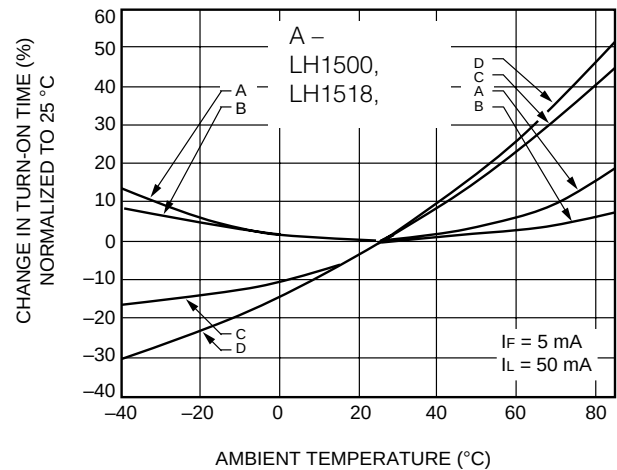
D. Turn-On Time vs. Temperature
