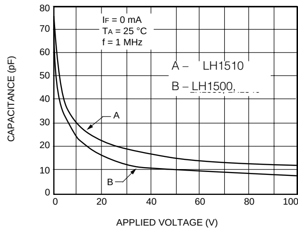
C. Switch Capacitance vs. Applied Voltage
