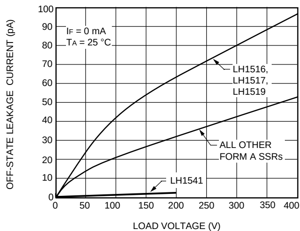
E. Leakage Current vs. Applied Voltage
