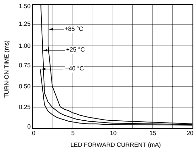
D. Turn-On Time vs. LED Current (LH1541)
