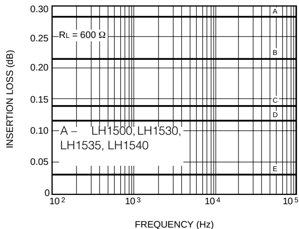
A. Insertion Loss vs. Frequency
