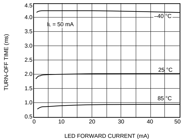
F. Turn-Off Time vs. LED Current (LH1504)
