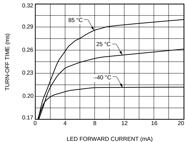
D. Turn-Off Time vs. LED Current (LH1525)
