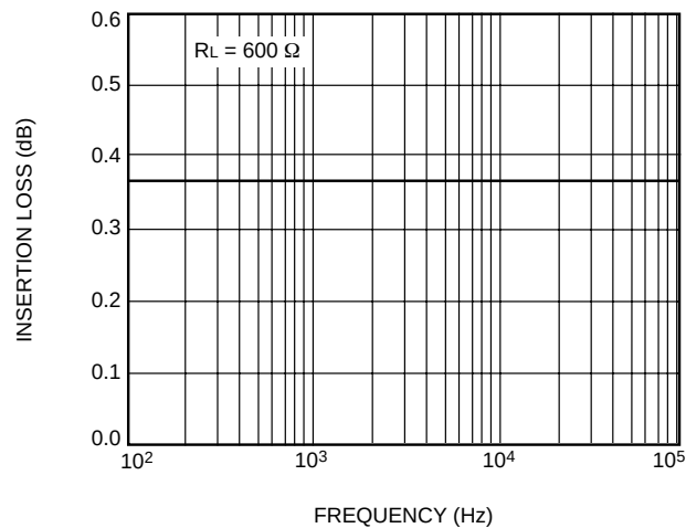
B. Insertion Loss vs. Frequency (LH1525)
