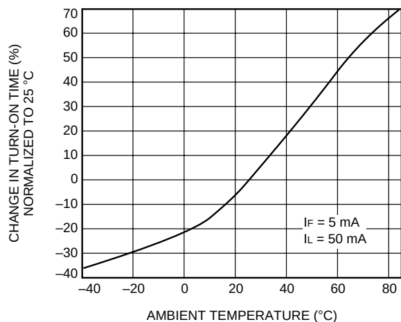
E. Turn-On Time vs. Temperature (LH1541)
