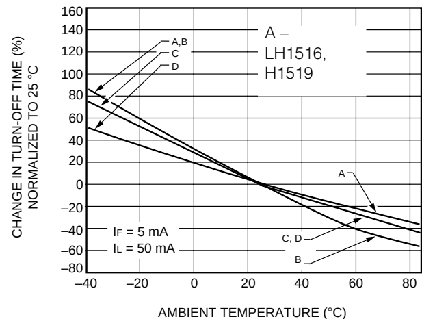
F. Turn-Off Time vs. Temperature
