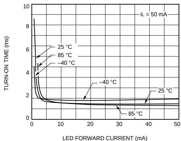
D. Turn-On Time vs. LED Current (LH1504)
