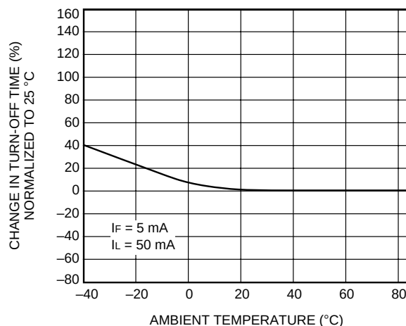
B. Turn-Off Time vs. Temperature (LH1541)
