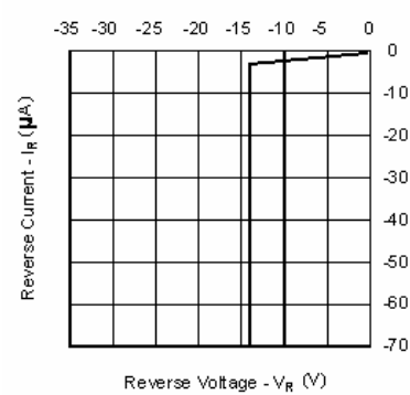
Figure 4-b: Reverse Voltage vs. Reverse Current – Blue and Green
