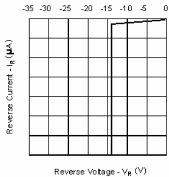
Figure 4-a: Reverse Voltage vs. Reverse Current – Red and Amber
