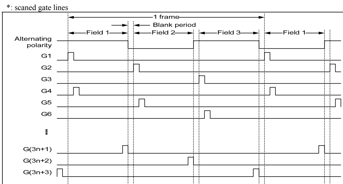
Figure 59 Gate output timing of 3-field interlaced scan
