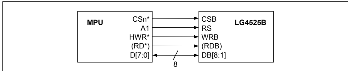
Figure 30 8-bit Interface
