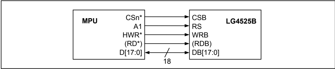
Figure 18 18-bit Interface
