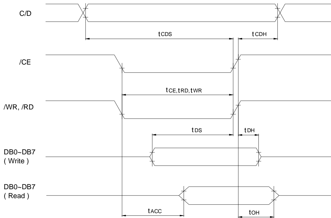
Fig.1 Bus Read/Write Timing
