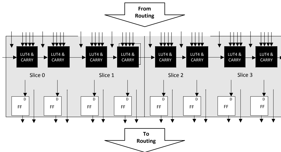
Figure 2.2. PFU Diagram
