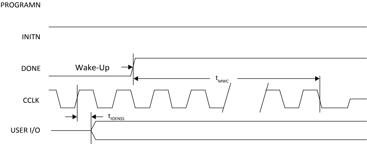
Figure 3.21. Wake-Up Timing
