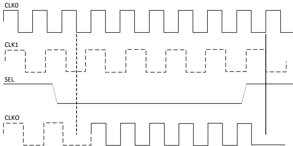
Figure 2.7. DCS Waveforms
