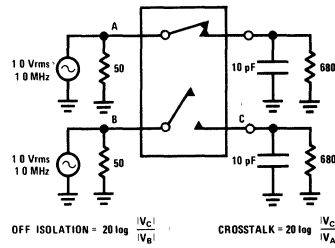
FIGURE 5. OFF Isolation and Crosstalk
