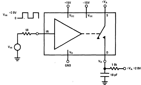
FIGURE 4. t_{ON} , t_{OFF} Test Circuit
