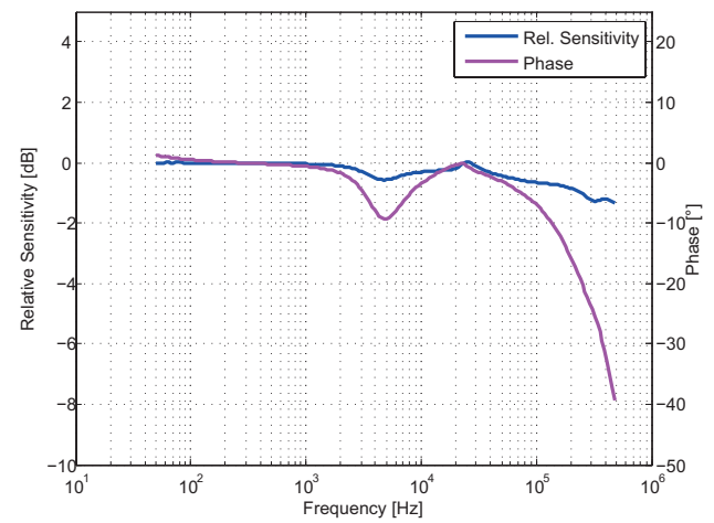
Figure 12: Frequency response
