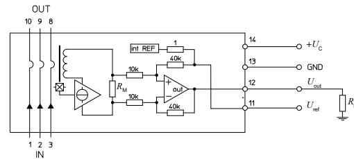
Figure 26: Test connection
