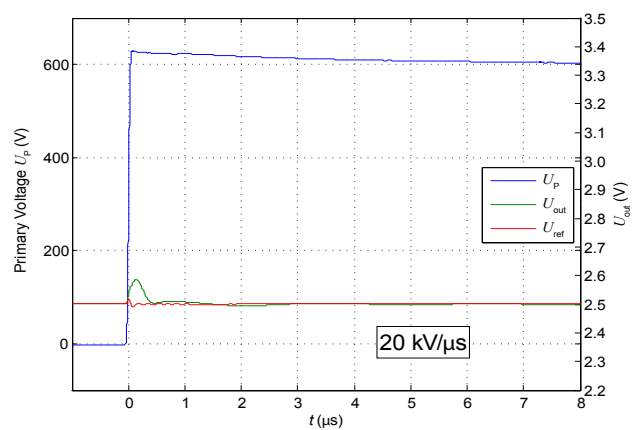
Figure 15: du/dt
