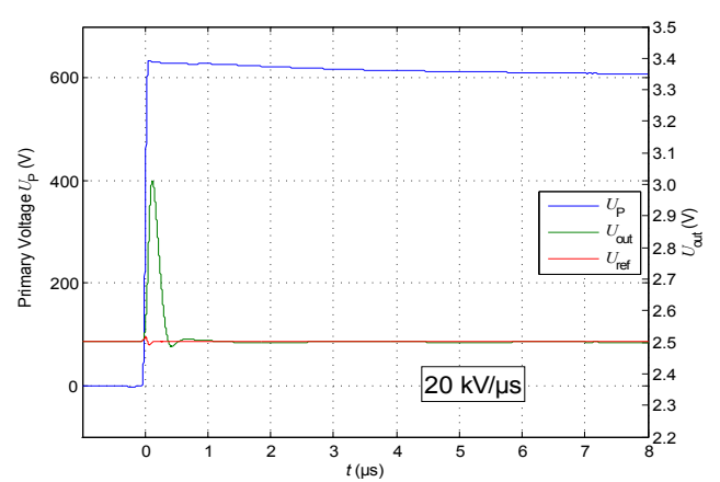
Figure 5: du/dt
