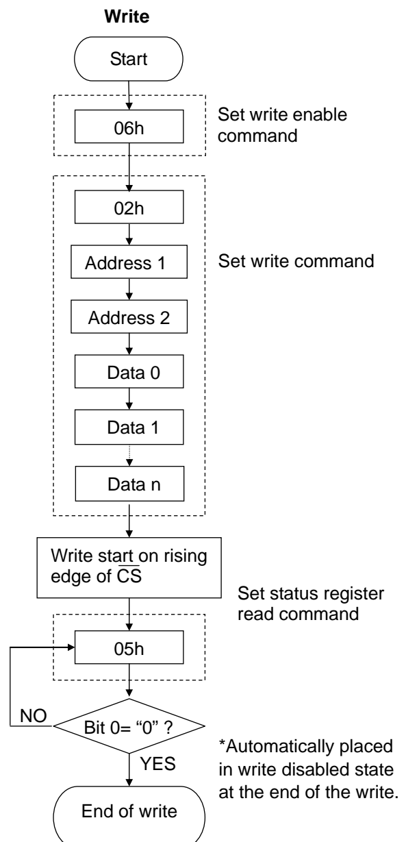
Figure 12 Write Flowchart
